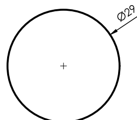
6178 Barra maciza Ø29mm 1,783 kg/m 4000 mm
