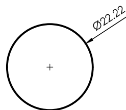
6176 Barra maciza Ø22,22mm 1,046 kg/m 4000 mm
