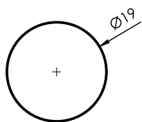
6175 Barra maciza Ø19mm 0,765 kg/m 4000 mm
